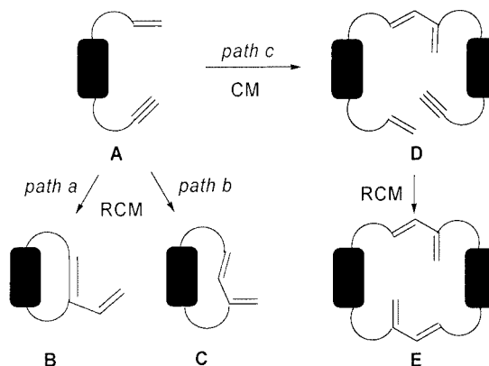
Scheme 1. Metathesis pathways of enynes
