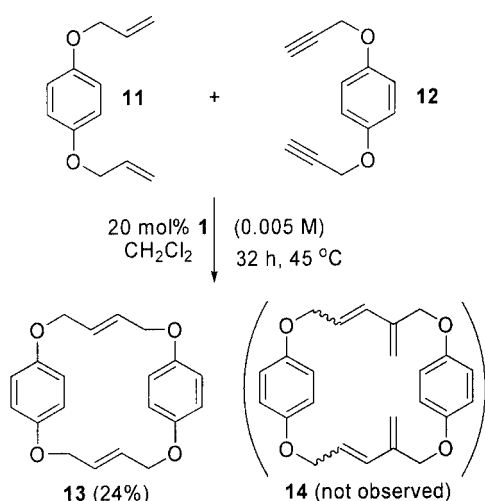
Scheme 2. Metathesis of a mixture of diene 11 and diyne 12
