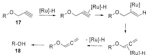
Scheme 5. A proposed mechanism for the deprotection of propargyl ethers
