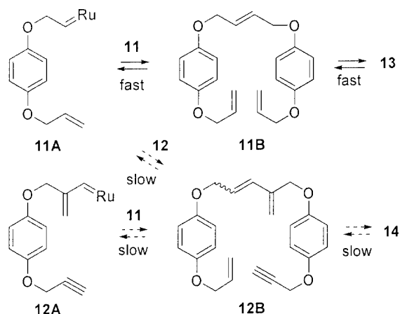
Scheme 3. Mechanism of cross metathesis of 11 and 12
