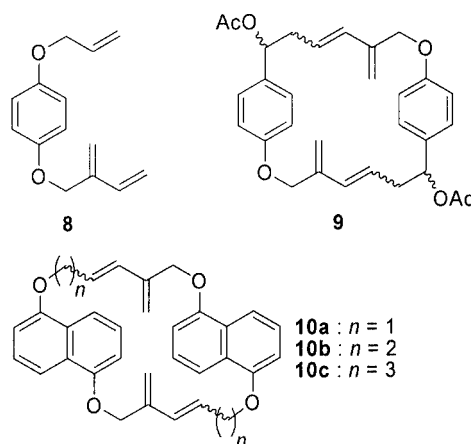
Figure 3. Enyne-metathesis products
