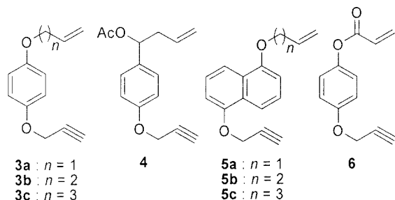
Figure 2. Enyne substrates
