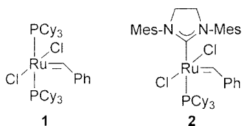
Figure 1. Grubbs' carbene ruthenium complexes
